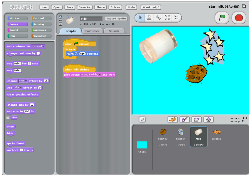
Figure 3. Screenshot of Brandy’s project, “star milk”
